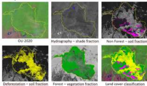
Figure 4. Classification of land cover classes for 2020 (hydrography in blue, non-forest in magenta, deforestation in yellow, and forest in green, respectively).
