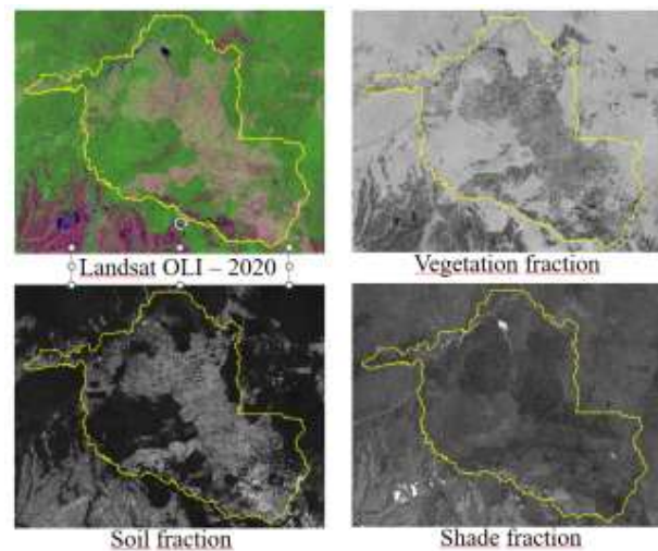
Figure 3. a) RGB color composite and b) vegetation, c) soil and d) shade fraction images derived from the OLI 2020 image mosaic.
