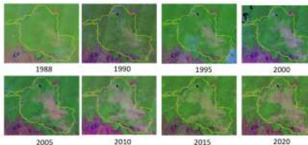
Figure 2. Landsat 5 TM (1988, 1990, 1995, 2000, 2005, 2010) and Landsat 8 OLI (2015-2020) images used in this work.
